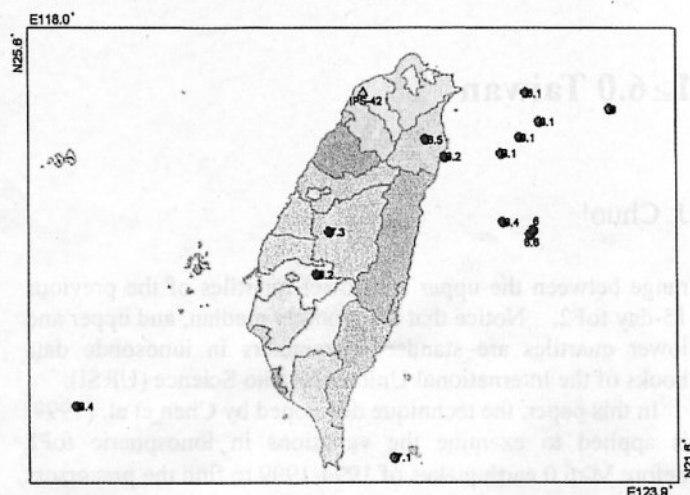
Figure 1. Locations of the ionosonde and the M \geq 6.0 earthquakes around Taiwan area during January 1994 - September 1999.
