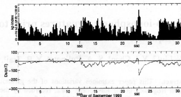
Figure 3. Variations of the geomagnetic indices Kp and Dst in September 1999. The horizontal axis represents the day of September 1999 in a UT coordinate and the SSC denotes the sudden storm commencement.
