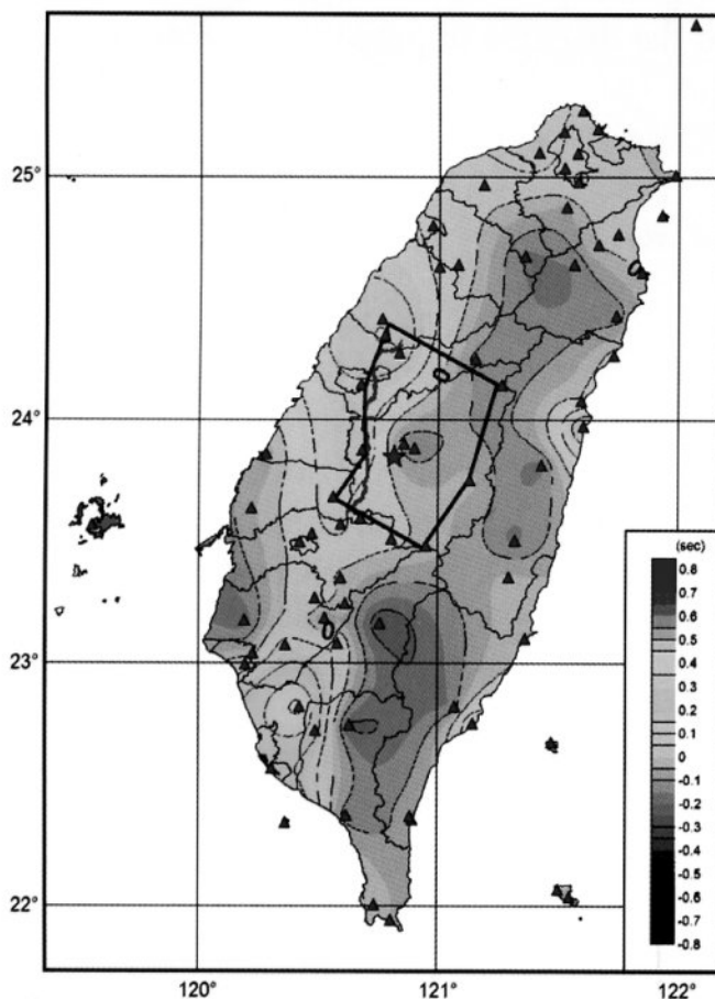
Mean residual time of P wave (1991-1993)
