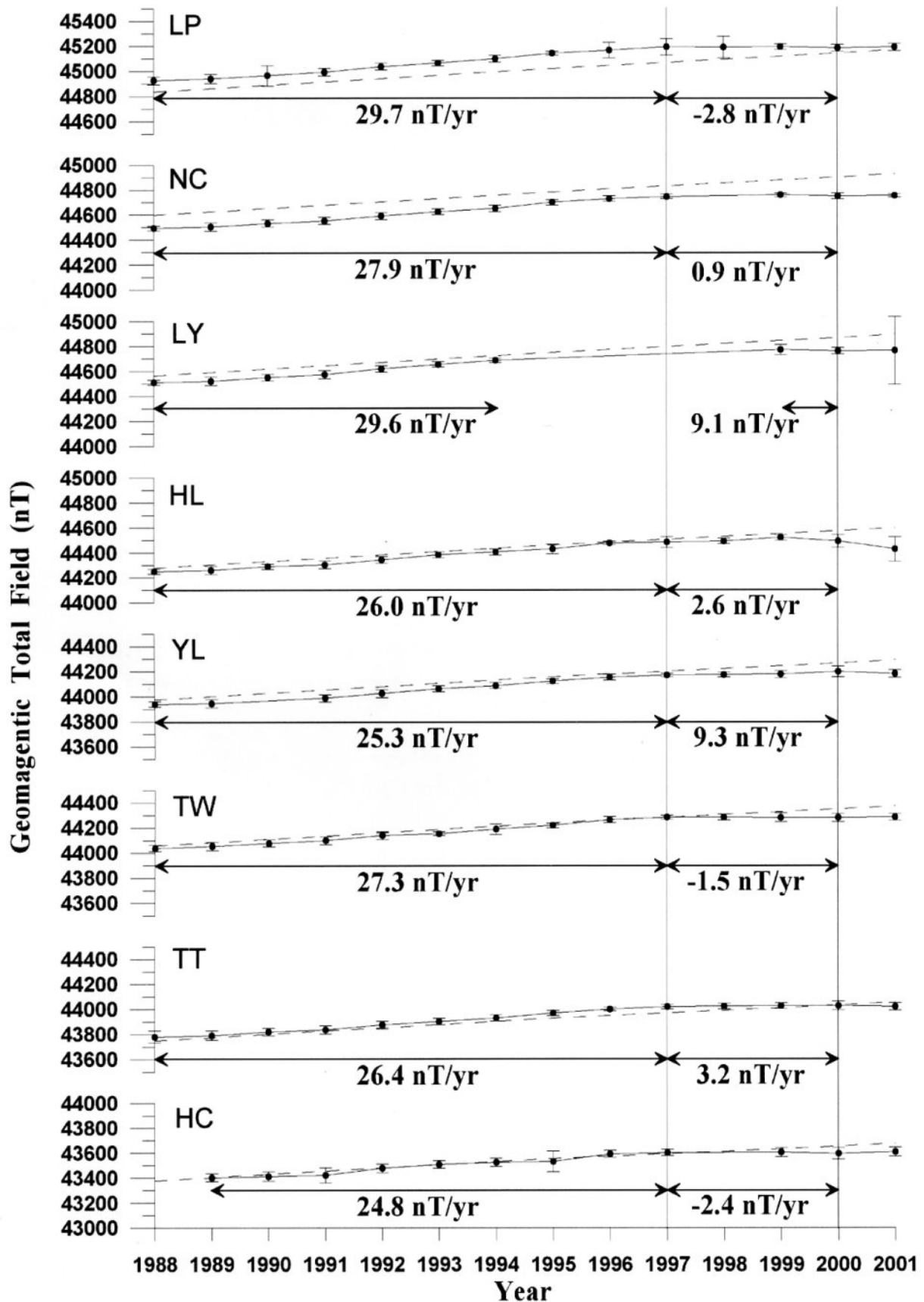
Fig. 5. Temporal variations of the geomagnetic total field during 1988-2001. The solid and dashed lines denote the yearly value of the observed and IGRF field, respectively. The error bars are the standard deviation of the yearly values. (After Chen et al. 2004).
