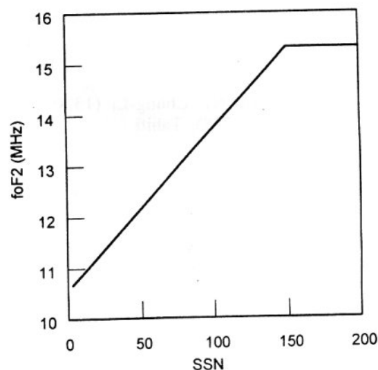
Fig.1. The simulated noon time foF2 at Chung-Li station during spring equinox.
