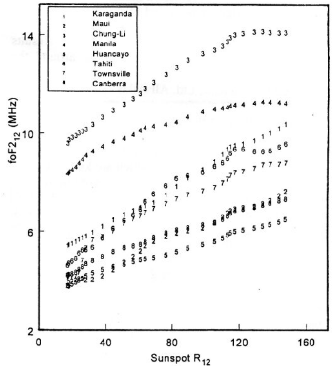
Fig. 3. Plots of foF2_{12} vs Sunspot R_{12} (1977/1-1979/6).
